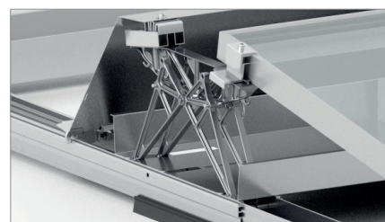
Support arrière 10°
