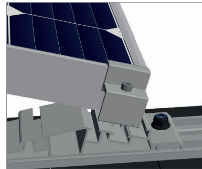
Detail front & back support
